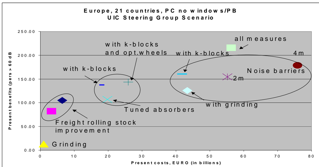
Figure 4.1: Main results of the STAIRRS project. The graph shows that solutions using composite brake blocks save considerable amounts of money in comparison to noise abatement with only noise barriers.
