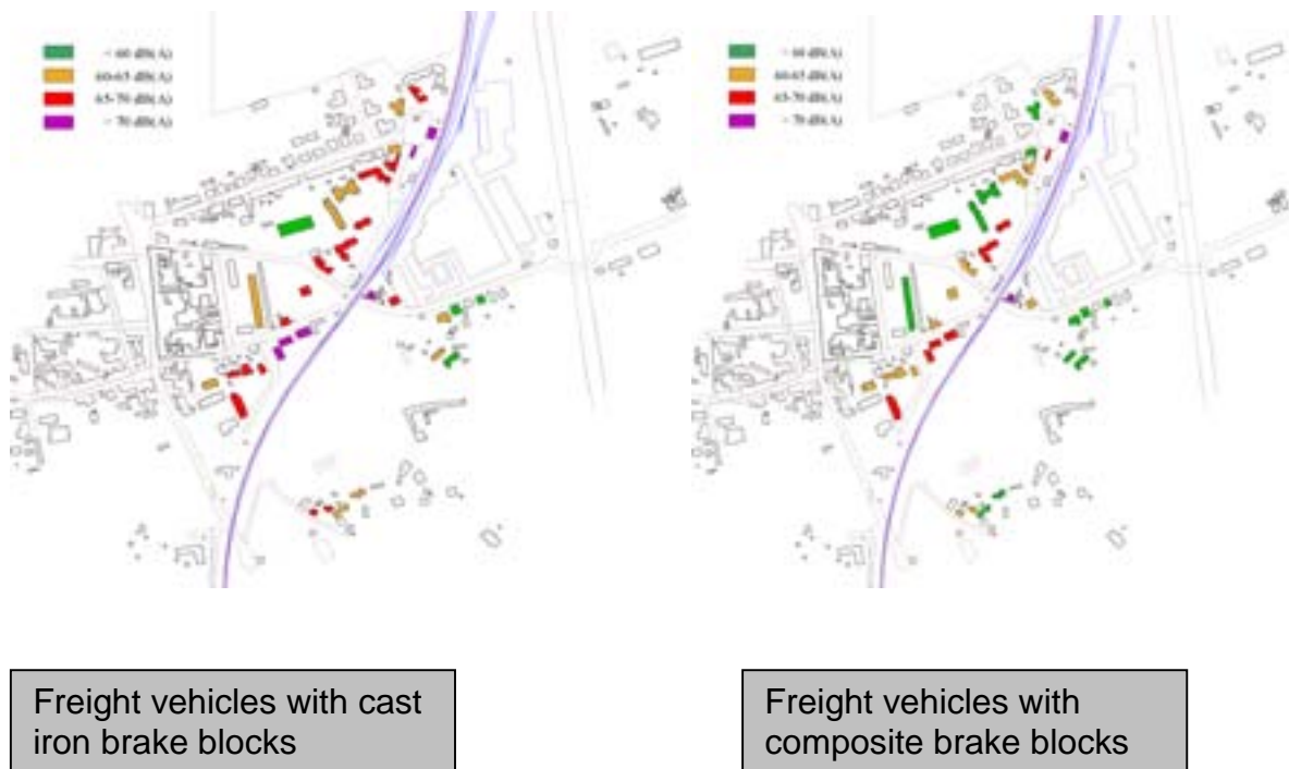
Figure A-4: Effects of composite brake blocks in freight vehicles on first floor noise levels in a typical residential situation in Italy (railway line from Genova to Roma). It is estimated that noise barrier requirements can be reduced by 30 % in this particular situation. Note that the highest noise levels (>70 dB(A), violet) are almost entirely eliminated and the second highest (65 – 70 dB(A), red) are considerably reduced with the introduction of composite brake blocks. On the other hand, there is a significant increase in buildings with low noise levels (<60 dB(A), green).
