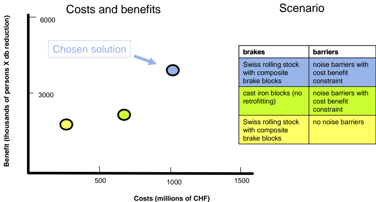
Fig. A-1: Railway noise abatement in Switzerland with and without composite brake blocks. Values are end cost estimates based on status of project in mid 2005. Combining rolling stock improvement with noise barriers increases cost-benefit ratio.
