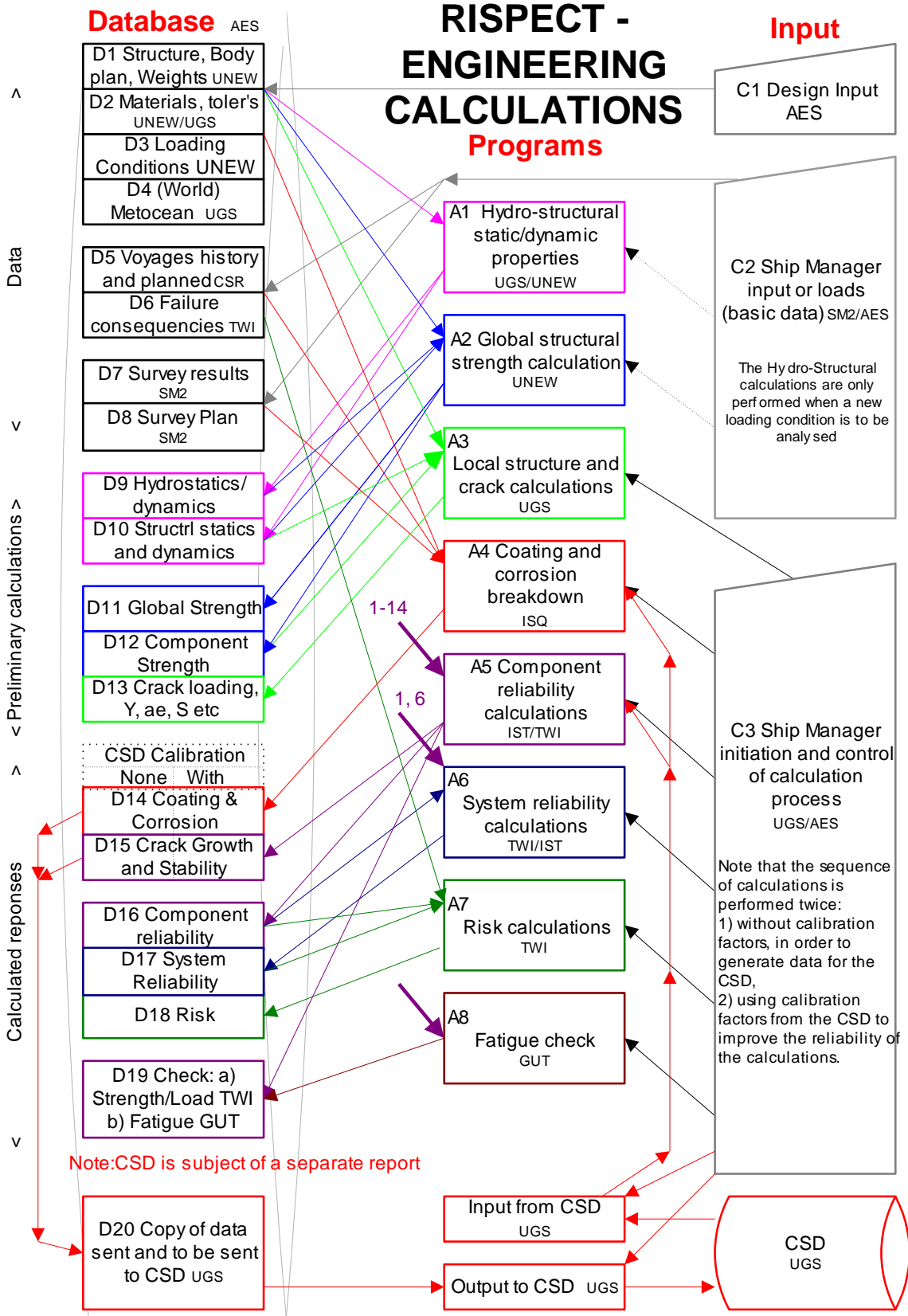
Figure 1.1 - RISPECT Engineering calculations – flow chart
