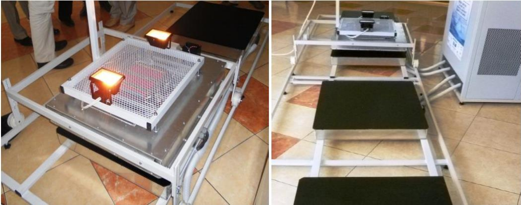
Figure 2 - Mock up for static and on-route inductive charging performance test and analysis
