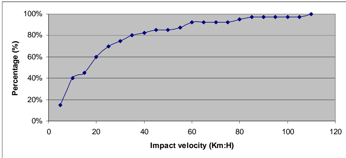
Figure 53: Scenario 9 - Cumulative frequency of impact velocity – Driver
