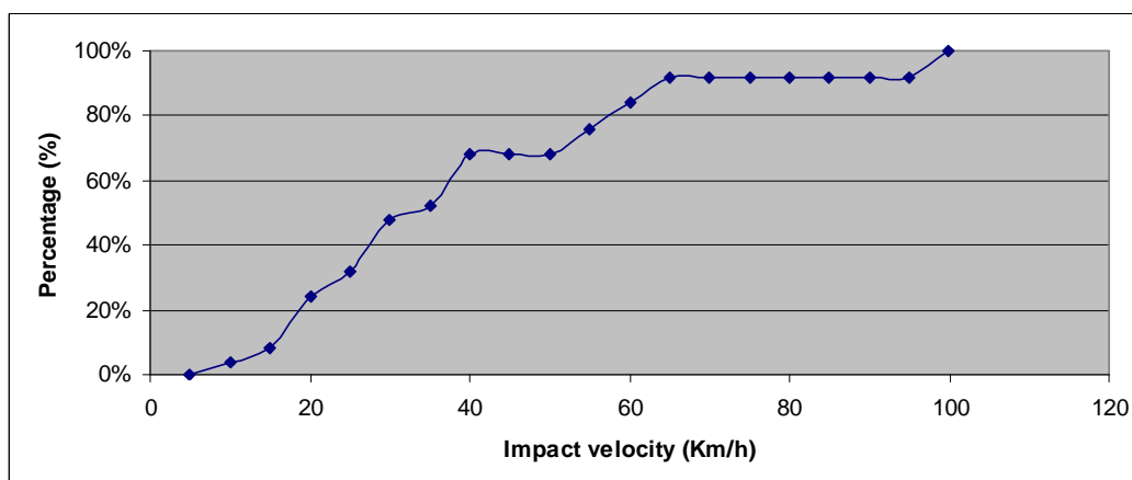
Figure 31: Scenario 5 - Cumulative frequency of impact velocity – Rider
