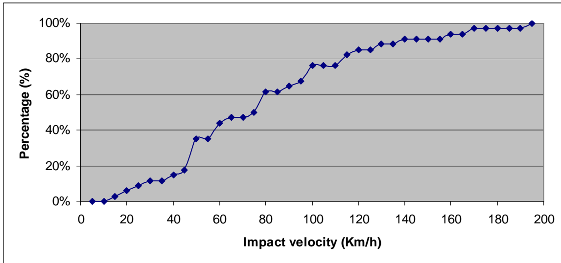
Figure 25: Scenario 3 - Cumulative frequency of impact velocity – Rider
