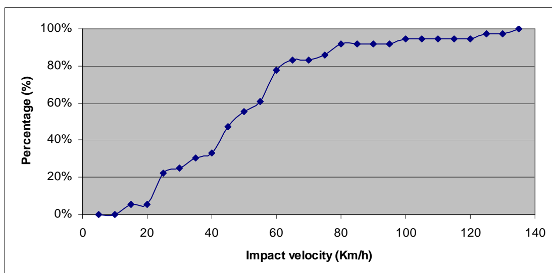
Figure 40: Scenario 7 - Cumulative frequency of impact velocity – Rider
