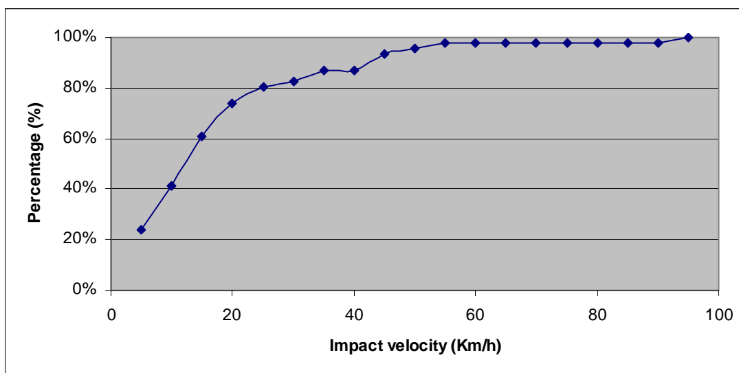
Figure 20: Scenario 2 - Cumulative frequency of impact velocity – Driver
