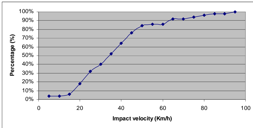
Figure 46: Scenario 8 - Cumulative frequency of impact velocity – Rider
