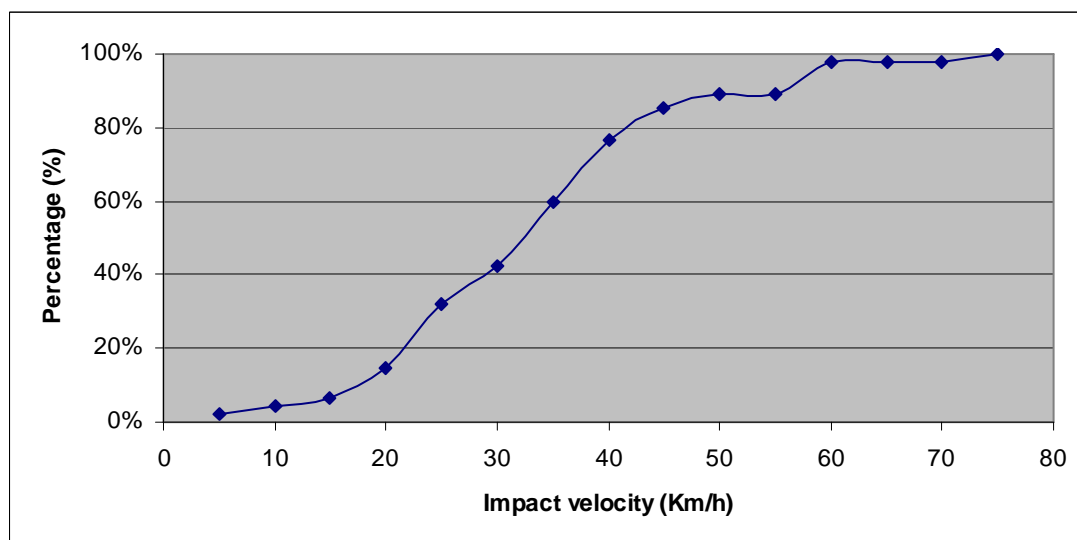
Figure 19: Scenario 2 - Cumulative frequency of impact velocity – Rider
