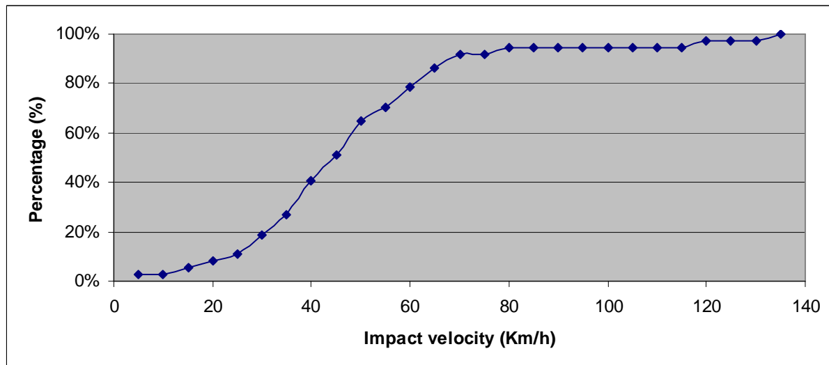
Figure 28: Scenario 4 - Cumulative frequency of impact velocity – Rider
