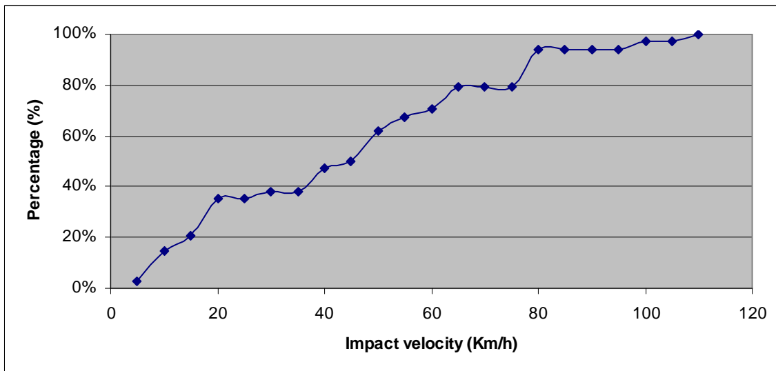
Figure 52: Scenario 9 - Cumulative frequency of impact velocity – Rider
