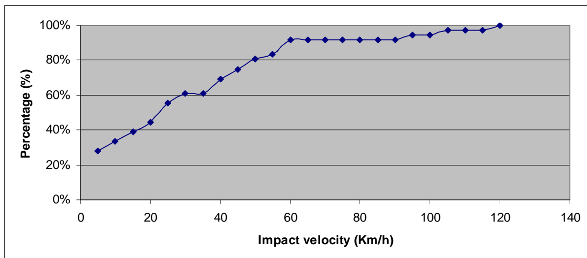
Figure 41: Scenario 7 - Cumulative frequency of impact velocity – Driver
