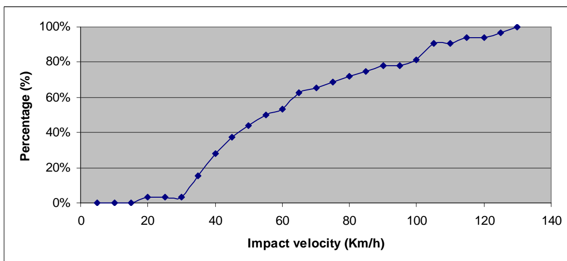
Figure 34: Scenario 6 - Cumulative frequency of impact velocity – Rider
