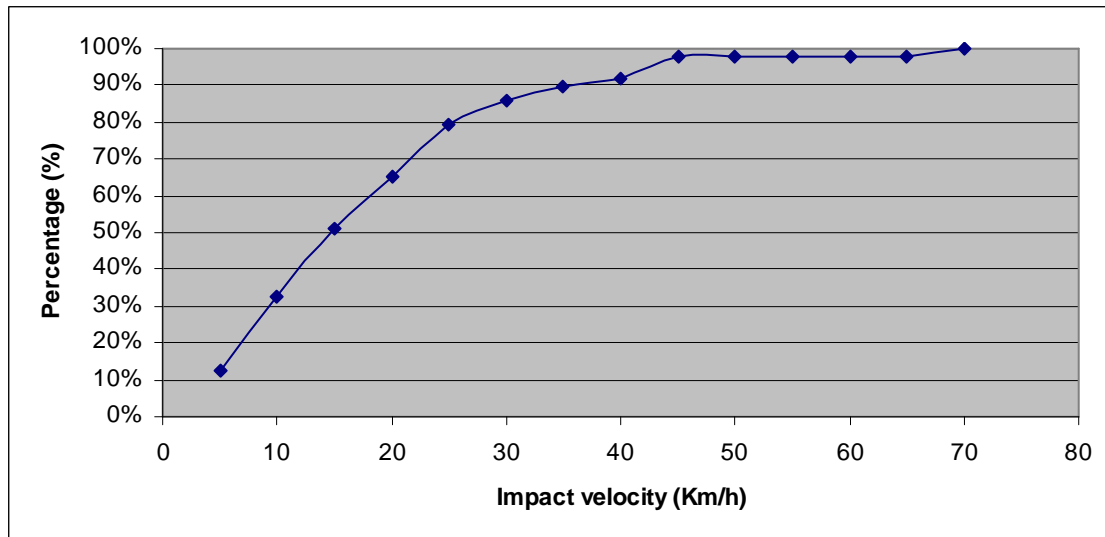
Figure 47: Scenario 8 - Cumulative frequency of impact velocity – Driver
