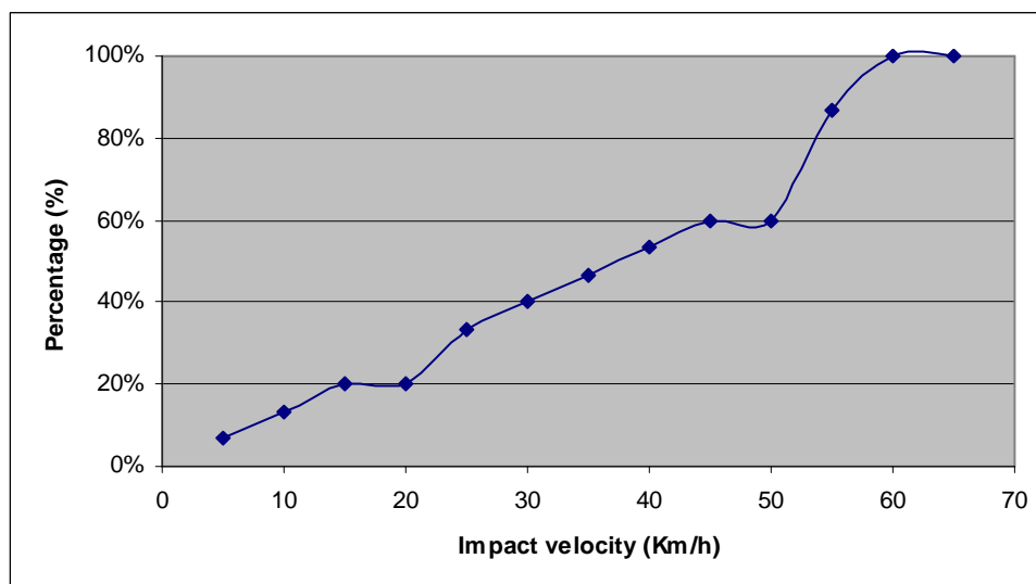
Figure 13: Scenario 1 - Cumulative frequency of impact velocity – Rider
