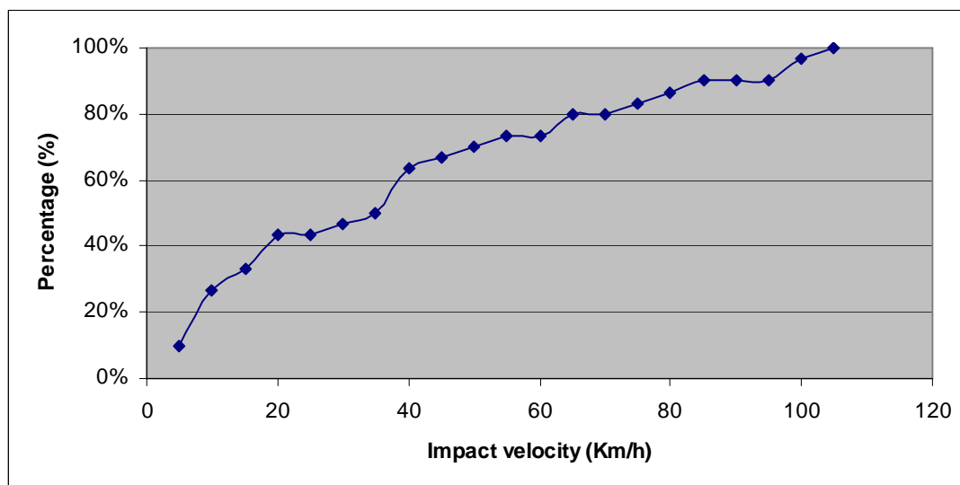
Figure 35: Scenario 6 - Cumulative frequency of impact velocity – Driver
