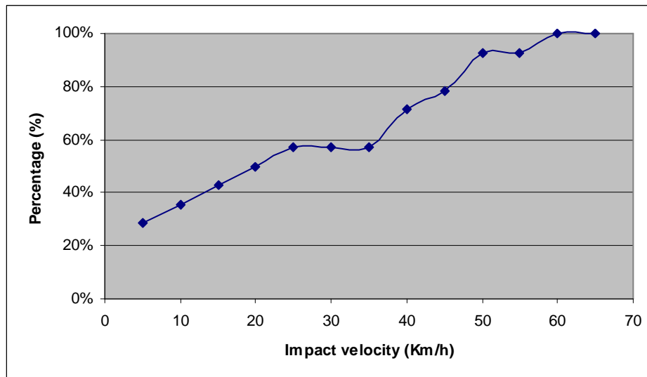
Figure 14: Scenario 1 - Cumulative frequency of impact velocity – Driver
