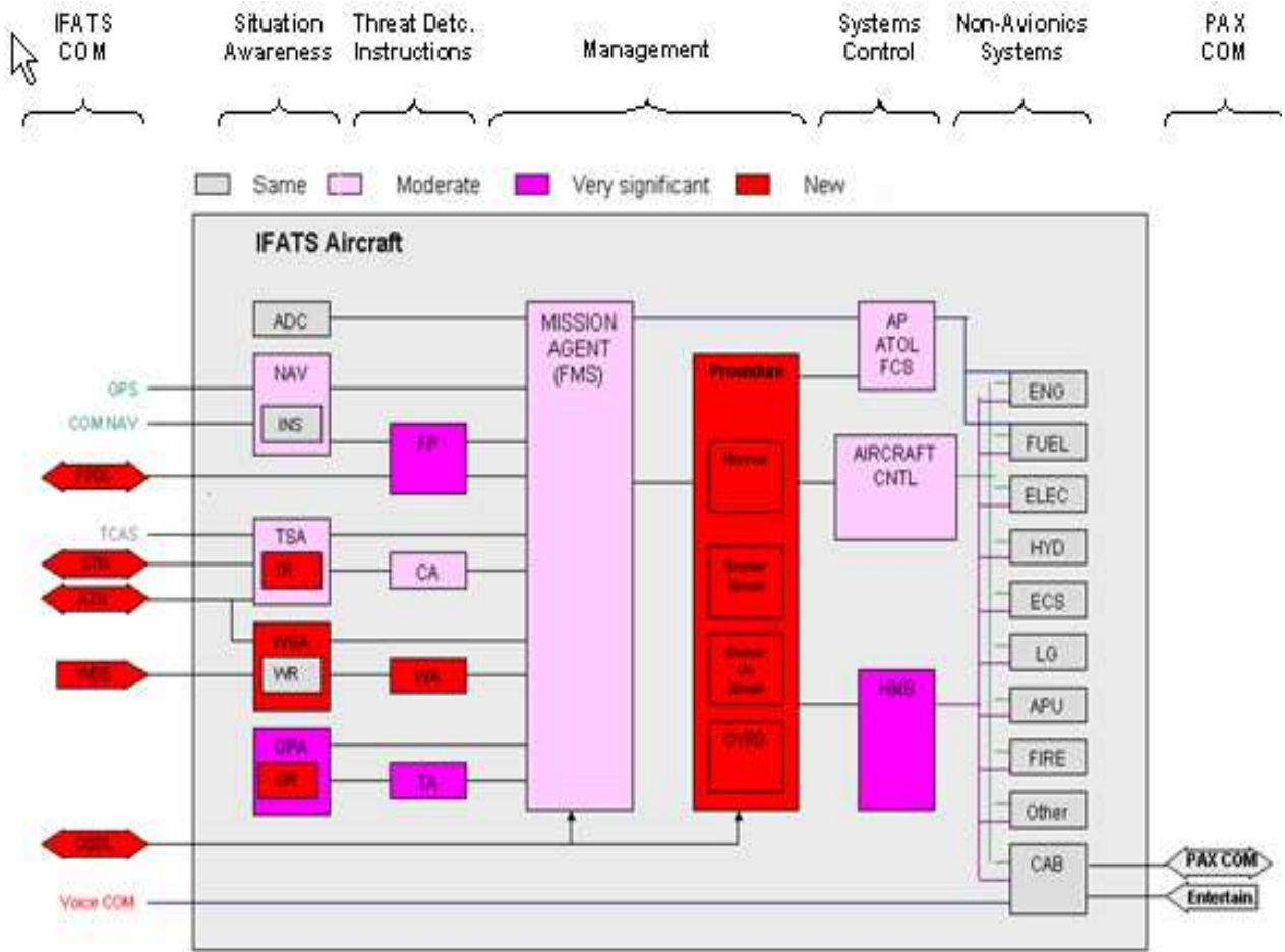
Figure 20 - IFATS Air Segment - Main functions
