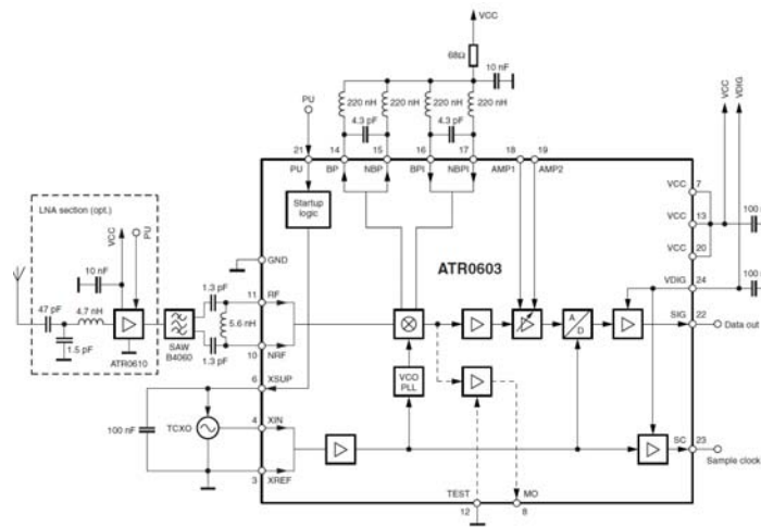
Figure 1-4: Atmel ATR0603 block diagram and suggested demo board components (www.atmel.com)
