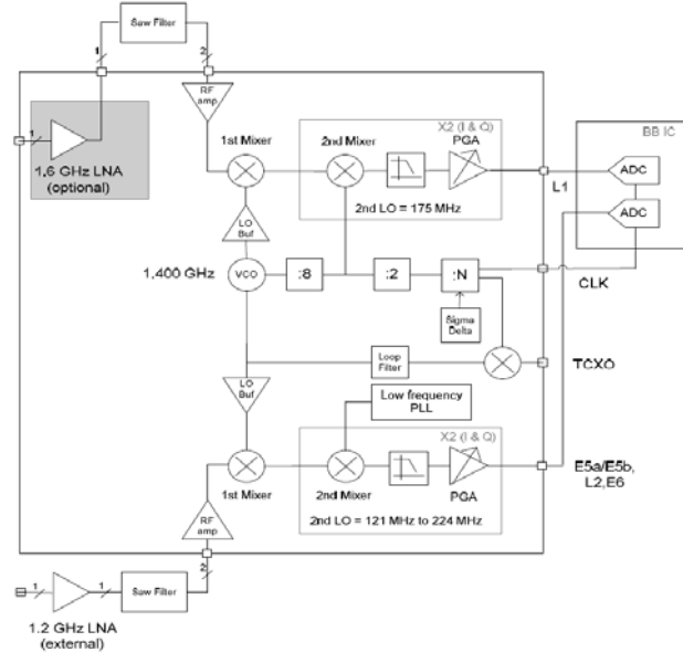
Figure 1-13: Functional diagram of the CI10612g
