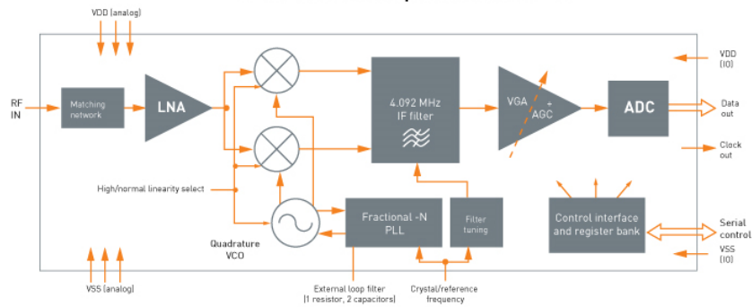
Figure 1-2: GNR1040 (www.stericsson.com)
