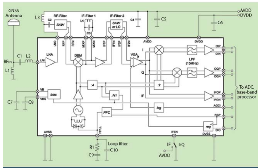
Figure 3-6: RF ASIC front end to be developed in the frame of the ARTUS project
