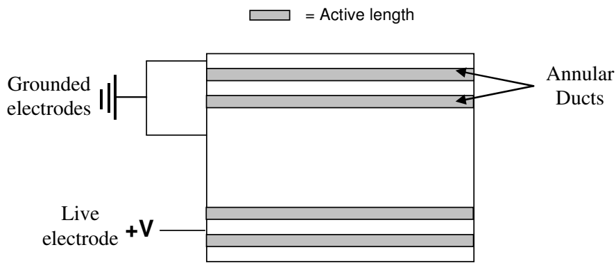
Figure 6.7.15: A multi-duct ER valve – Ducts can be arranged in series of parallel.
