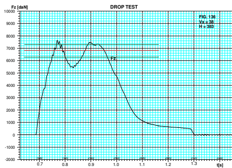
Fig.1 The classical characteristic for limit landing parameters; F_z (daN) - vertical force versus time t (s)
