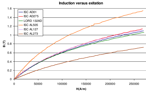
Figure 6.6.4 : B-H curve of different magnetic fluids
