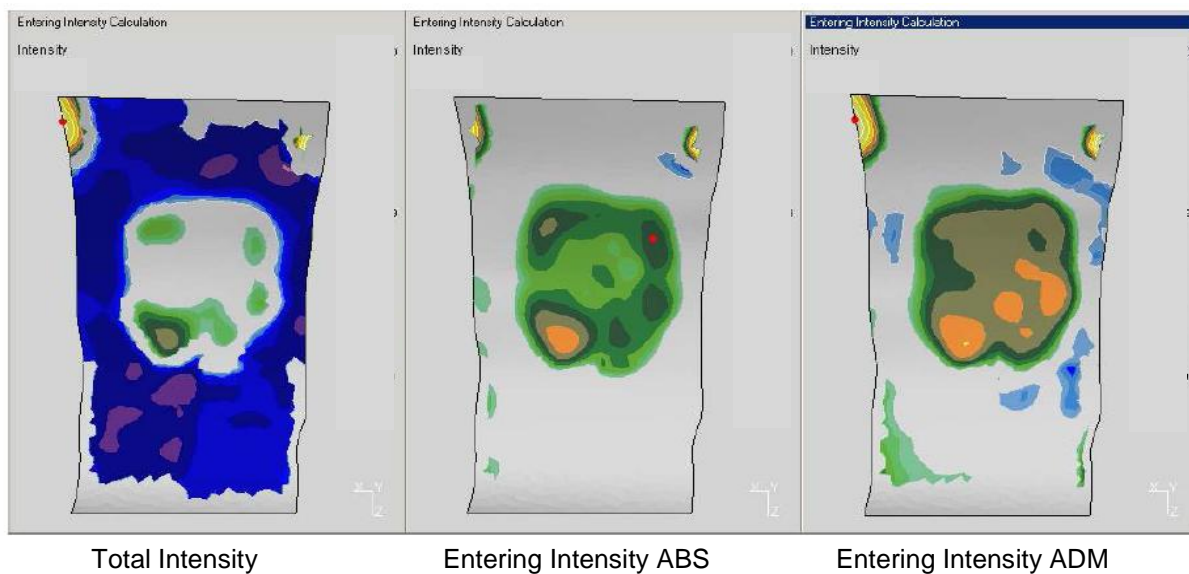
Figure 28: Example of estimation of absorption and entering intensity (window)
