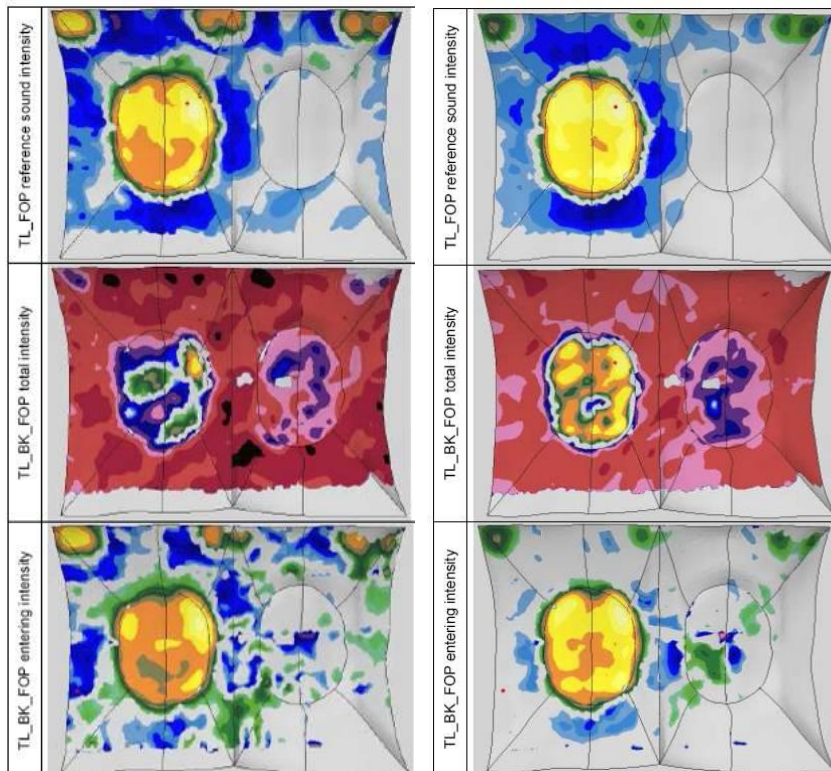
Figure 20: Entering intensity in the 1kHz octave band (left) and 2kHz octave band (right)
