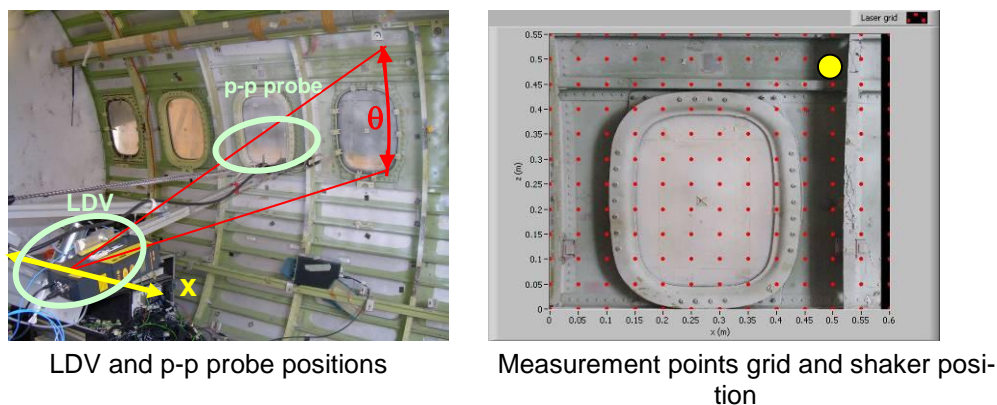
Figure 5: Test set-up
