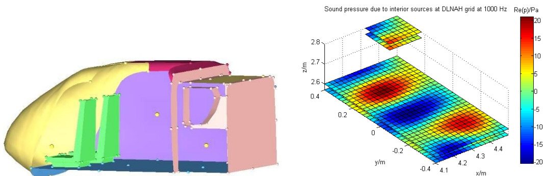
Figure 24: Location of additional sources for simulation of additional sources in phase (left) and pressure field at DLA-NAH array due to the additional sources in the cabin
