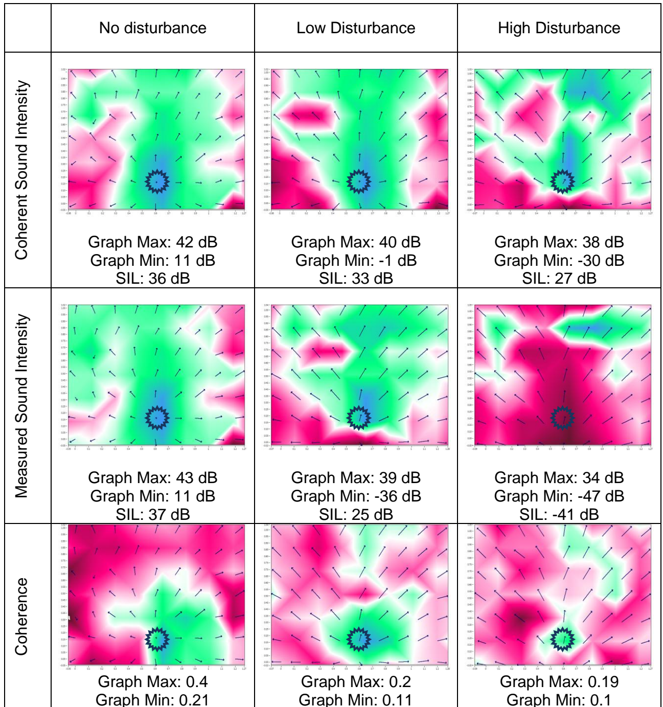
Figure 7: Coherent intensity as a function of the level of disturbance. Sound Intensity in the frequency range of 1000-2000 Hz. Stimulus and disturbances: uncorrelated Gaussian white noise. The symbol identifies the geometric position of the piezoelectric shaker.
