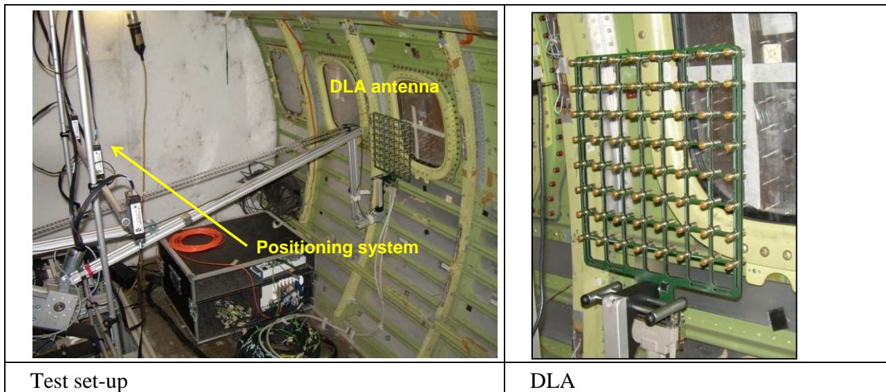
Figure 12: DLA installation
