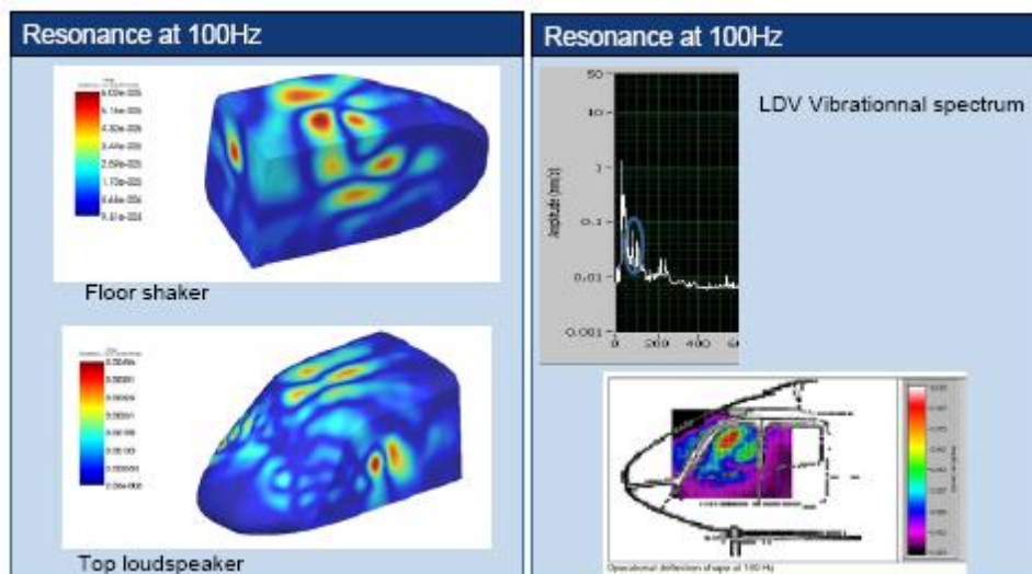
Figure 37: Reconstructed velocity field at 100 Hz
