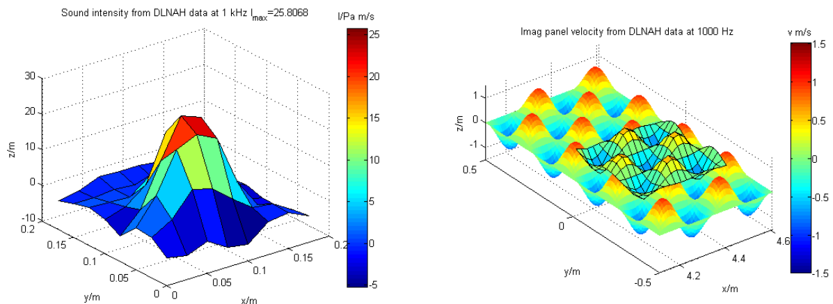
Figure 25: Reconstructed intensity from the DLA-NAH tool from B&K
