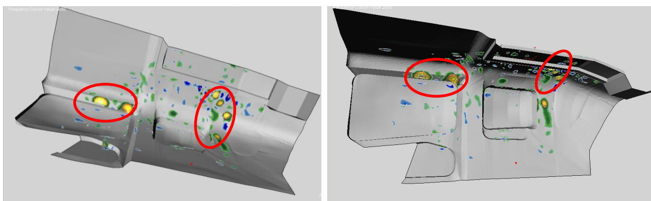
Figure 41: Intensity mapping at 2000Hz - view from the bottom and from the side of the cabin
