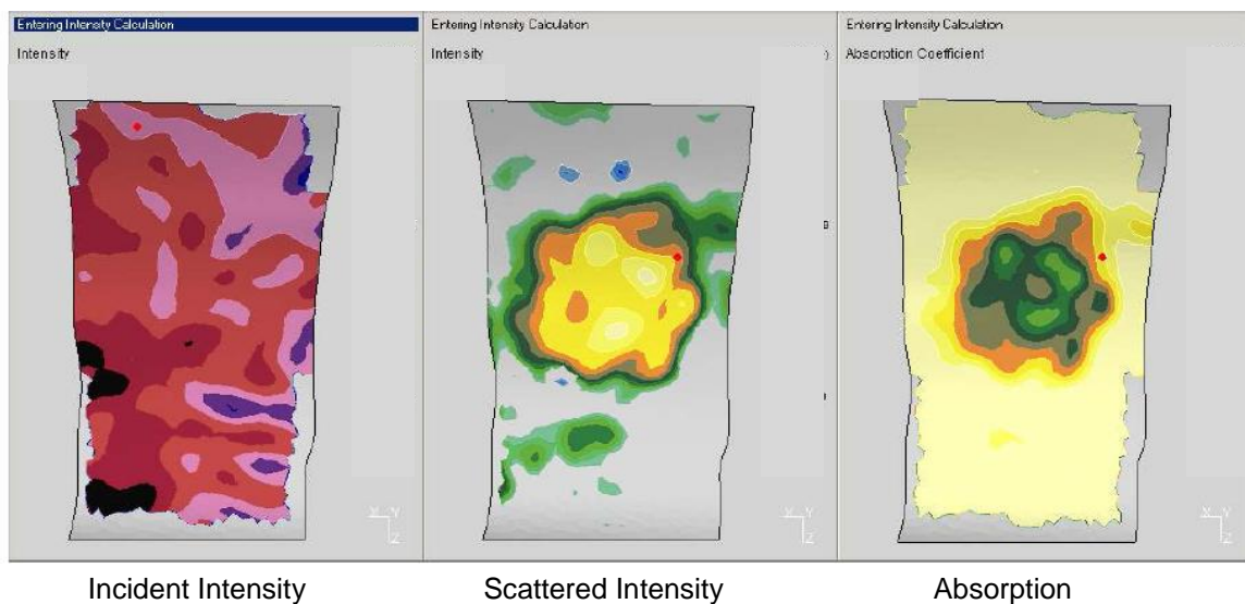
Figure 27: Measurement sequence for the rear window
