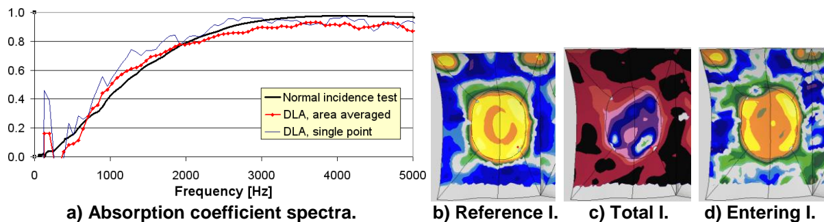
Figure 2: Extraction of the Entering Intensity. Green-yellow contours: Outward intensity. Blue-red: inward intensity. Contour interval: 2 dB. All maps show data for a single octave band with the same threshold level.
