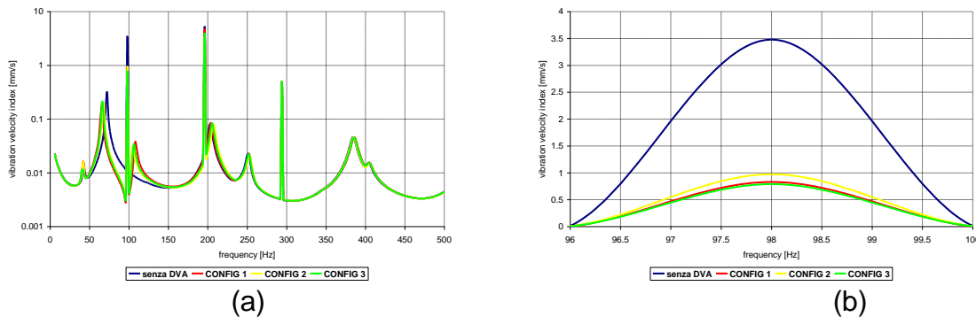
Figure 16: Results in terms of vibration velocity index for symmetric load and DVA tuned at 98 Hz (blue: without DVA, yellow, red, green: DVA in different configurations)
