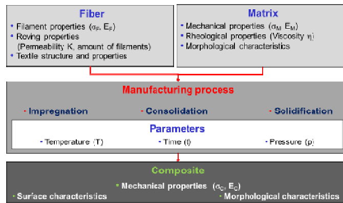
Figure 1a. Basics of composite manufacturing
