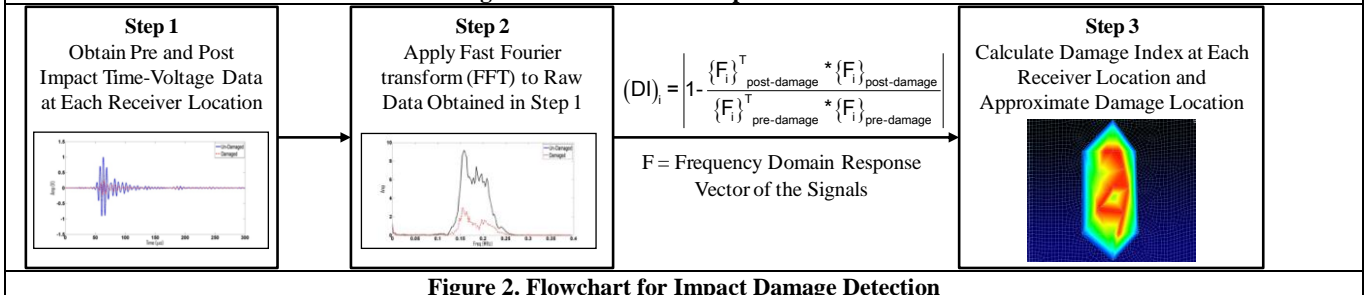
Figure 2. Flowchart for Impact Damage Detection
