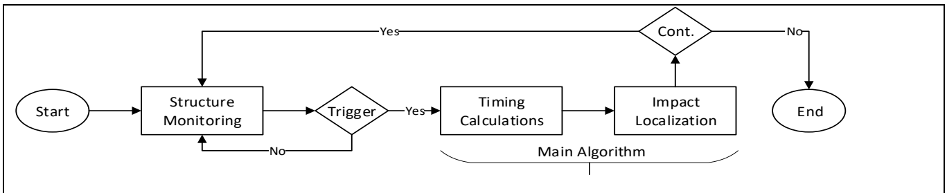
Figure 1. Workflow for Impact Localization
