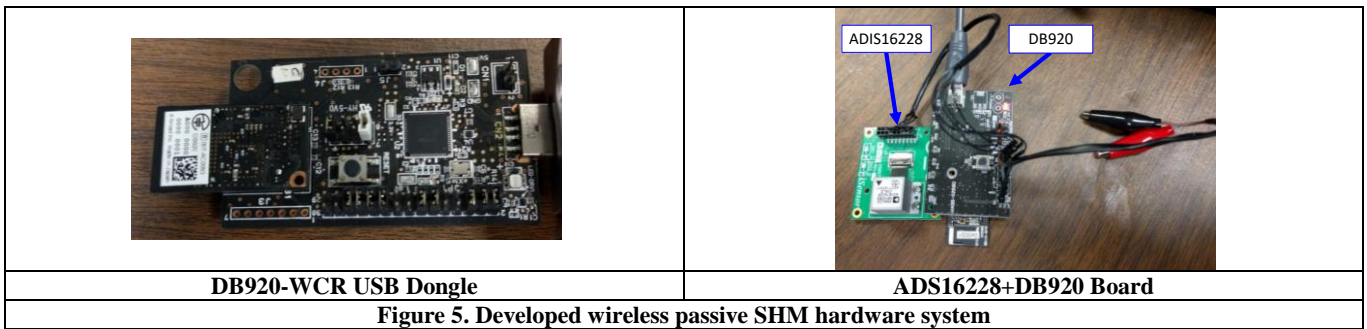
Figure 5. Developed wireless passive SHM hardware system
