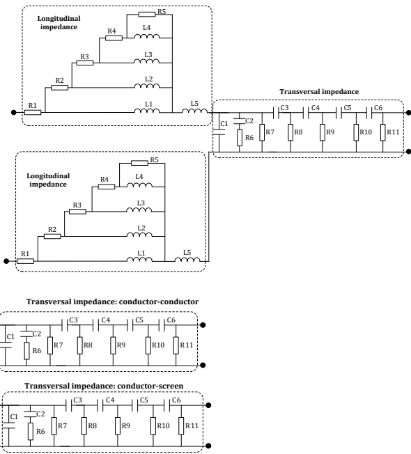
Longitudinal and transversal impedance models
