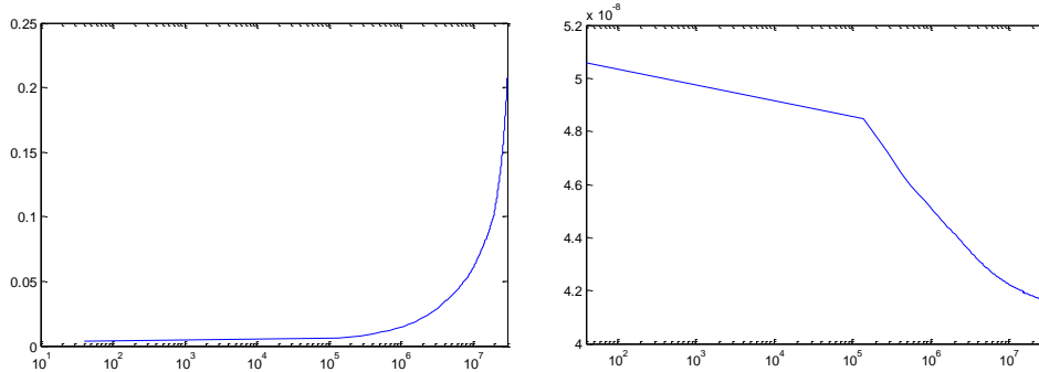
Calculated values of RI (Ohm) and LI (H) in the range 40 Hz-30 MHz from the measurements performed with the Agilent 4294A impedance analyzer. Short Circuit test
