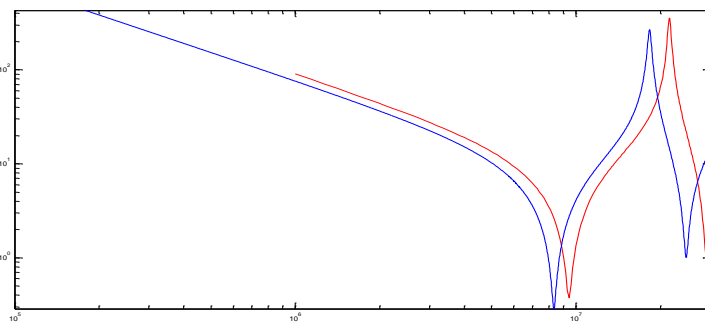
Three conductors in open circuit.
