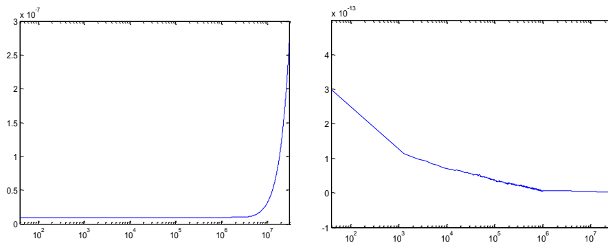
Calculated values of Gtc-s (1/Ohm) and Ctc-s (H) in the range 40 Hz-30 MHz from the measurements performed with the Agilent 4294A impedance analyzer. Open Circuit test
