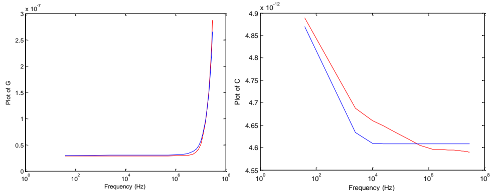
Rtc-c and Ctc-c. Red = experimental values. Blue = values fitted by means of the GA algorithm.
