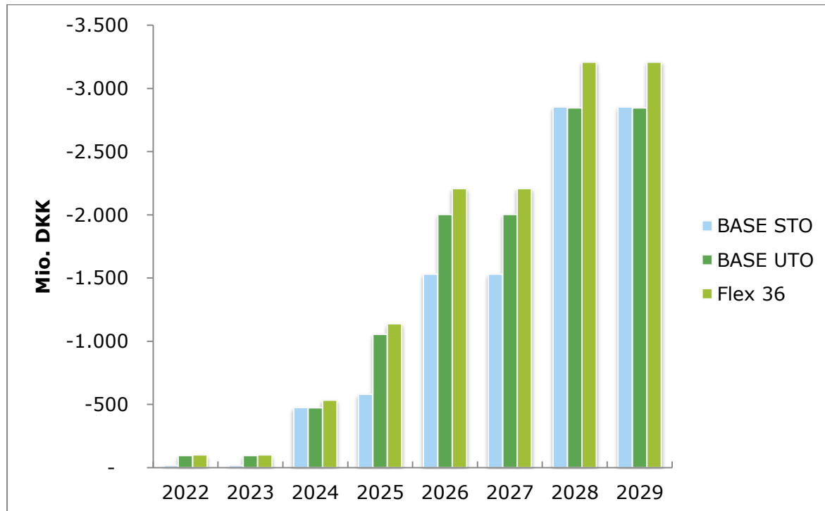
Figure 14: Investment CAPEX, 2022-2029
