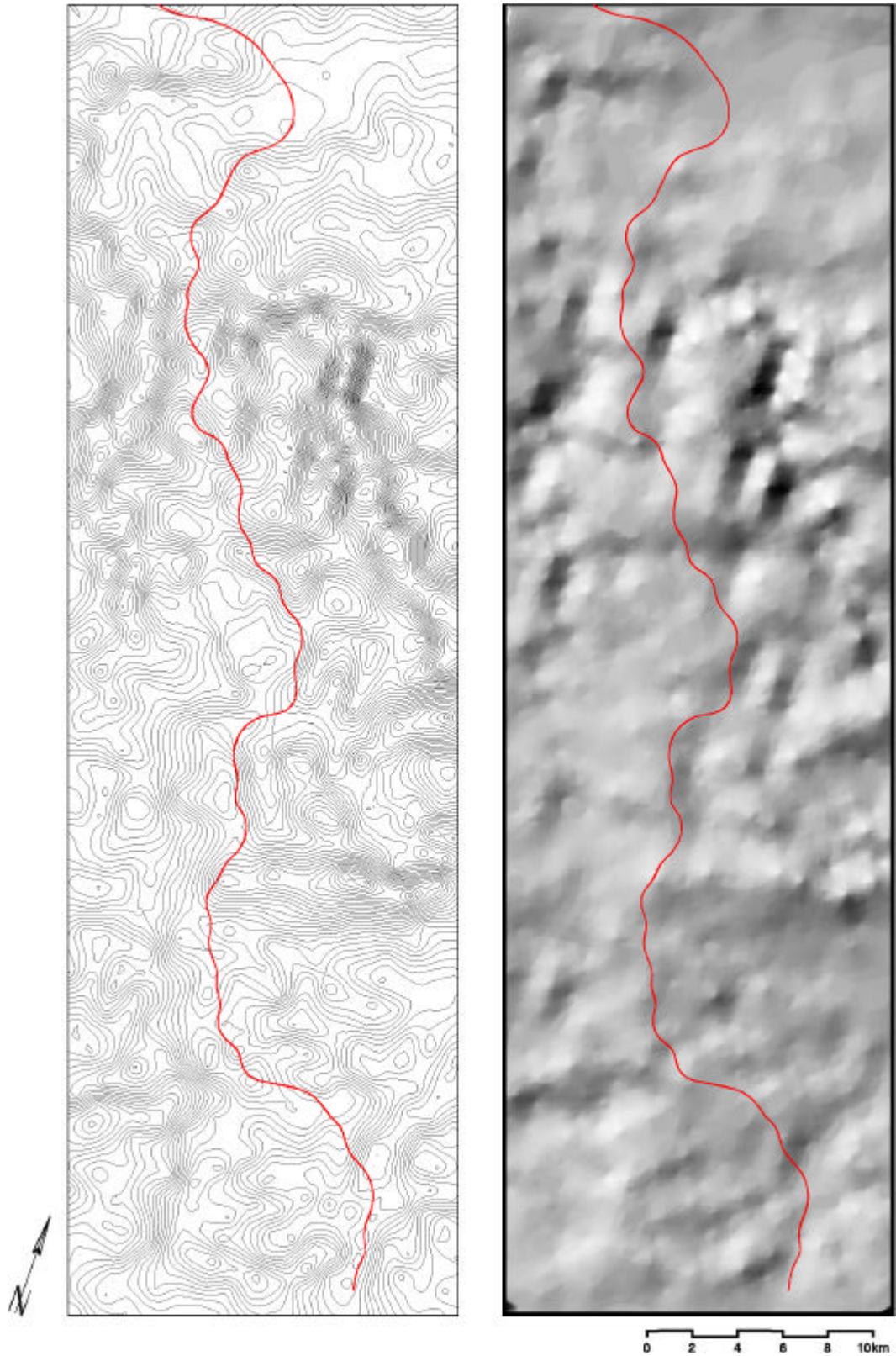
Figure 2c: A45 section and DTM C (1000 x 1000 m grid): 10 m contour lines (left), relief (right).
