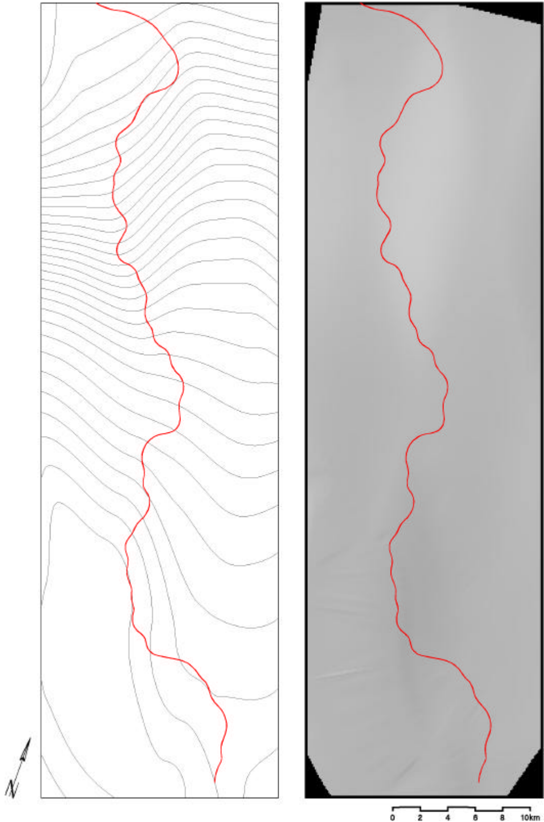
Figure 2e: A45 section and DTM E (9 x 15 km grid): 10 m contour lines (left), relief (right).
