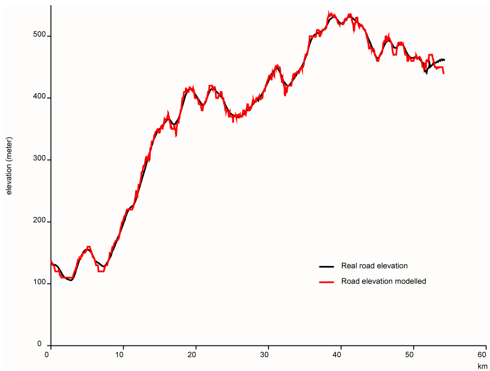
Figure3. Real elevation profile and modelled elevation profile (DTM 1:25,000).
