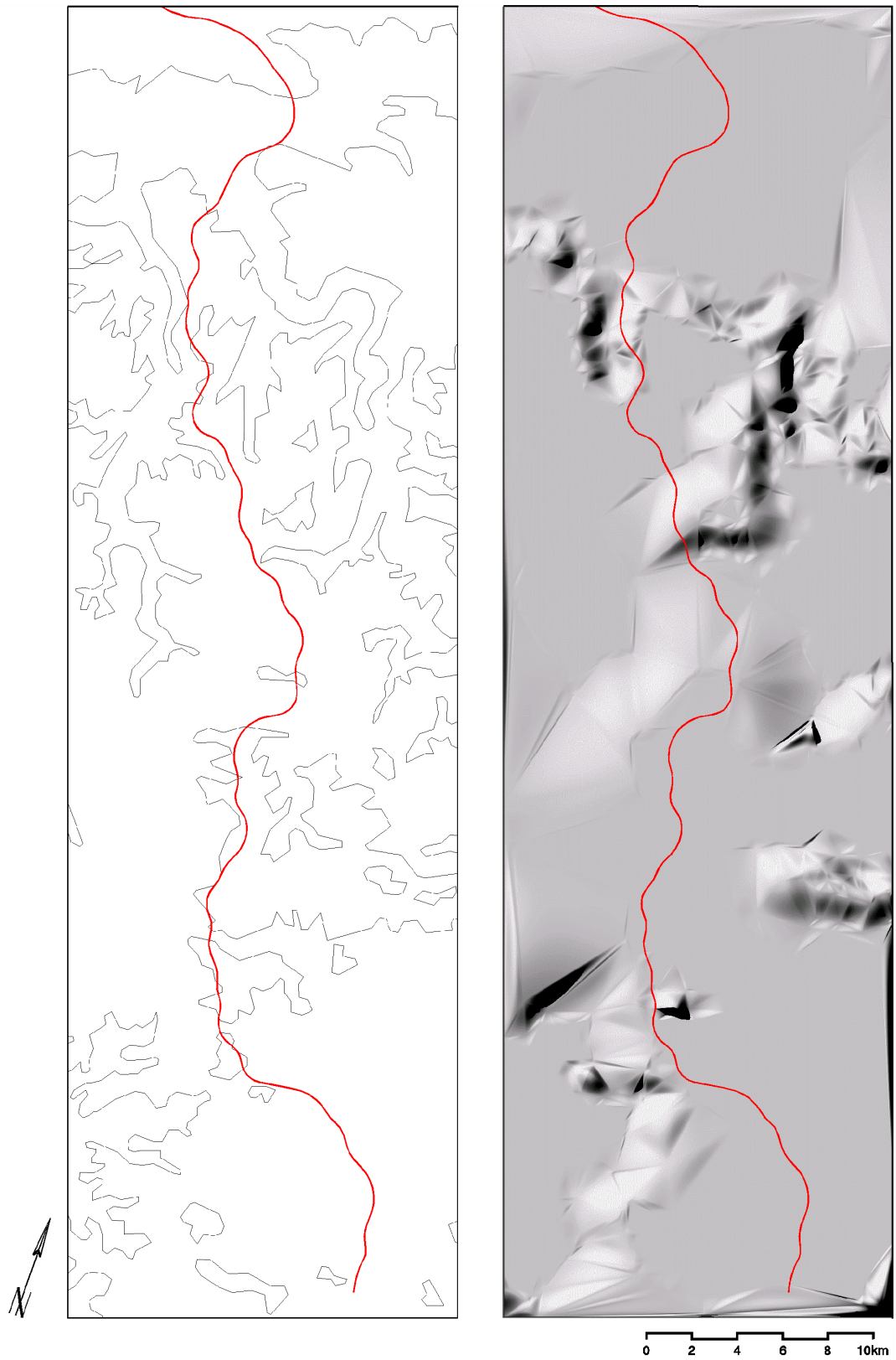
Figure 2d: A45 section and DTM D (1:1,000,000): original contour lines (left), relief (right).
