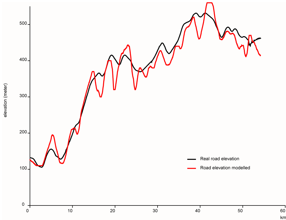
Figure 4. Real elevation profile and modelled elevation profile (DTM 30").
