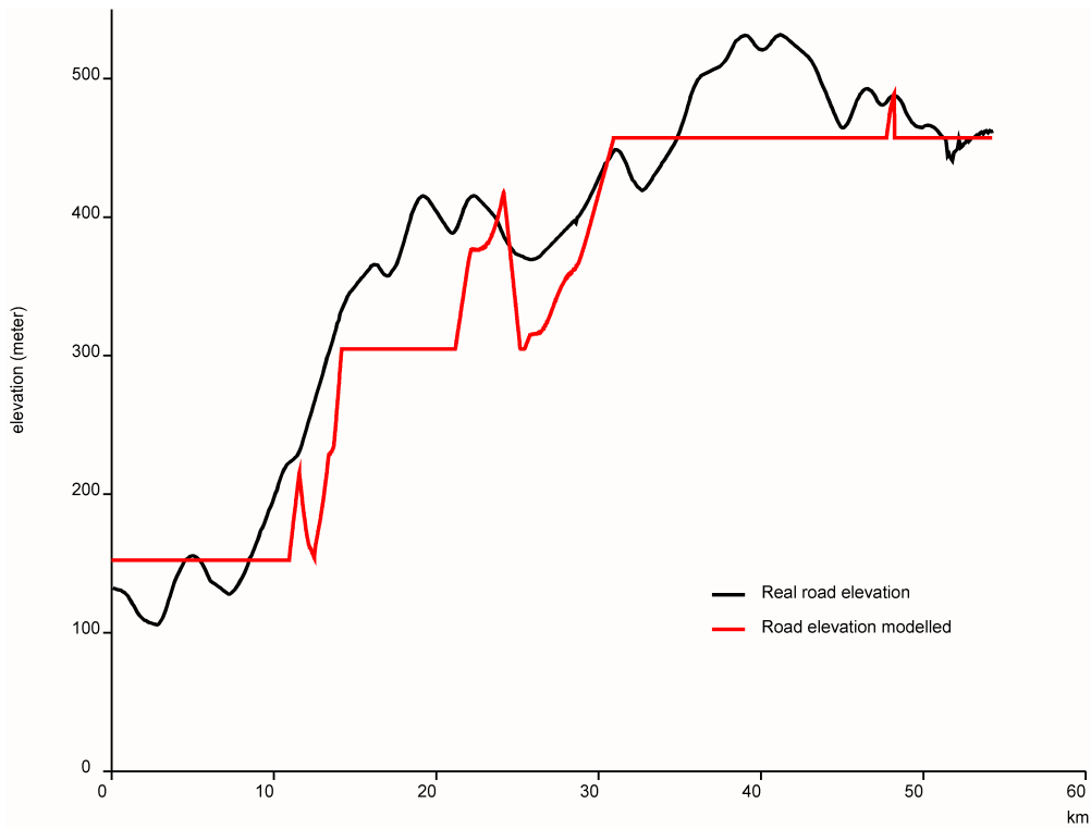
Figure 5: Real elevation profile and modelled elevation profile (DTM: DCW, 1:1,000,000).
