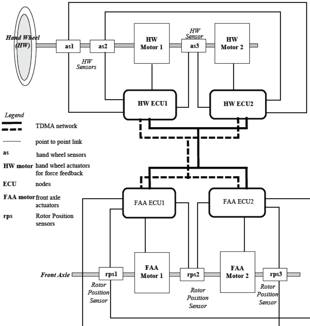
Figure 29: X-by-wire architecture from Brite-EuRam 111 Program, X-by-wire
