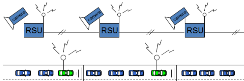
Figure 4: Mixed traffic in platoons, as experimentally tested during the SPITS project in The Netherlands
