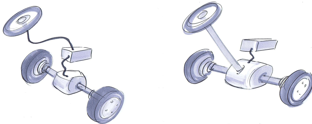
Figure 28: Schematics for X-by-wire (left side, no mechanical steering column) and software control (right side, using the power steering actuator with the mechanical steering column in parallel)
