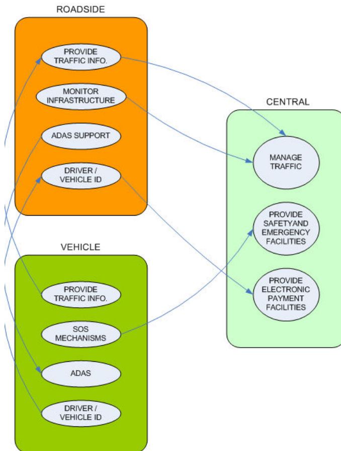
Figure 47: Physical and communications architecture for scenario 2
